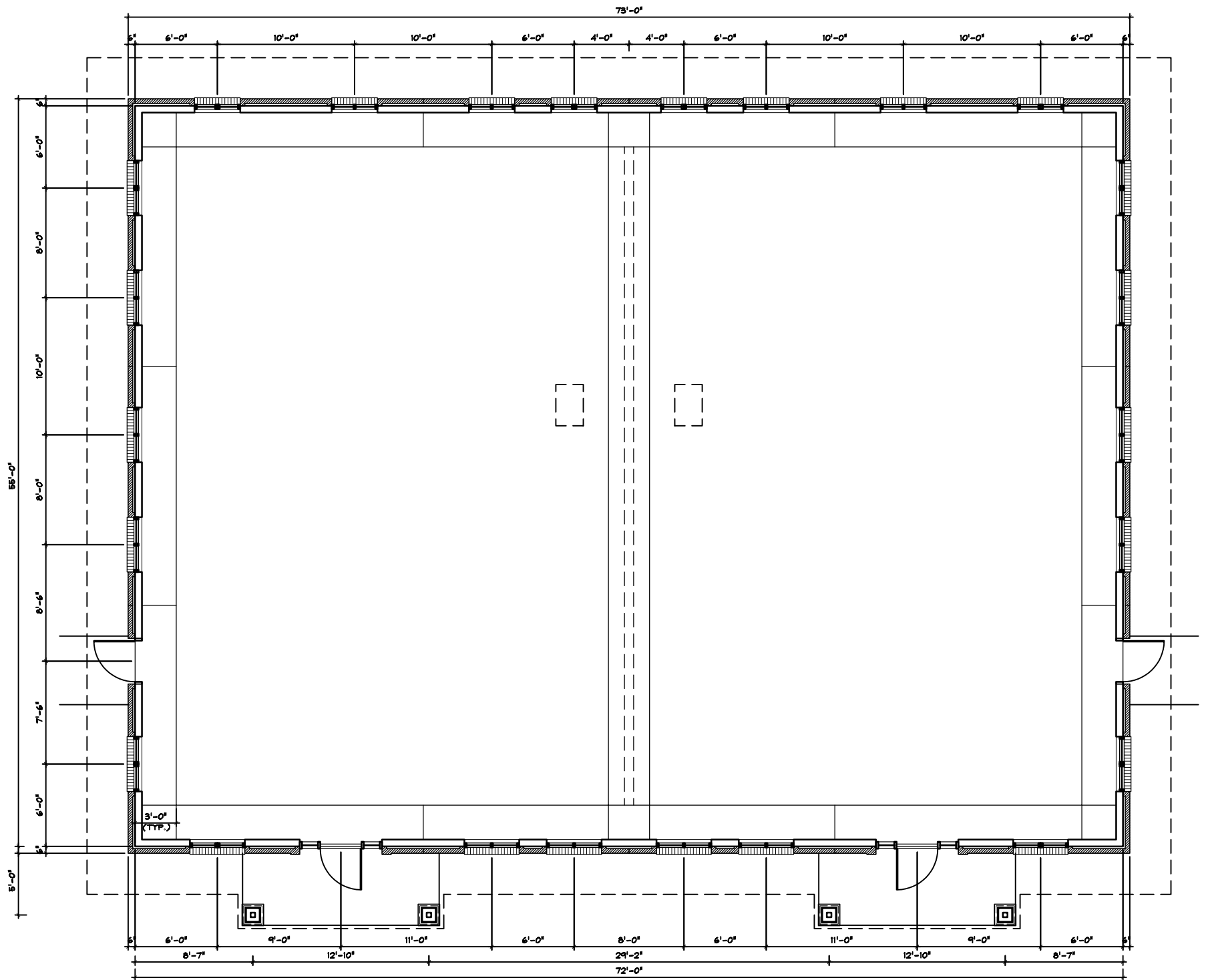
BUILDING C PLAN (3,888 SQUARE FEET)
