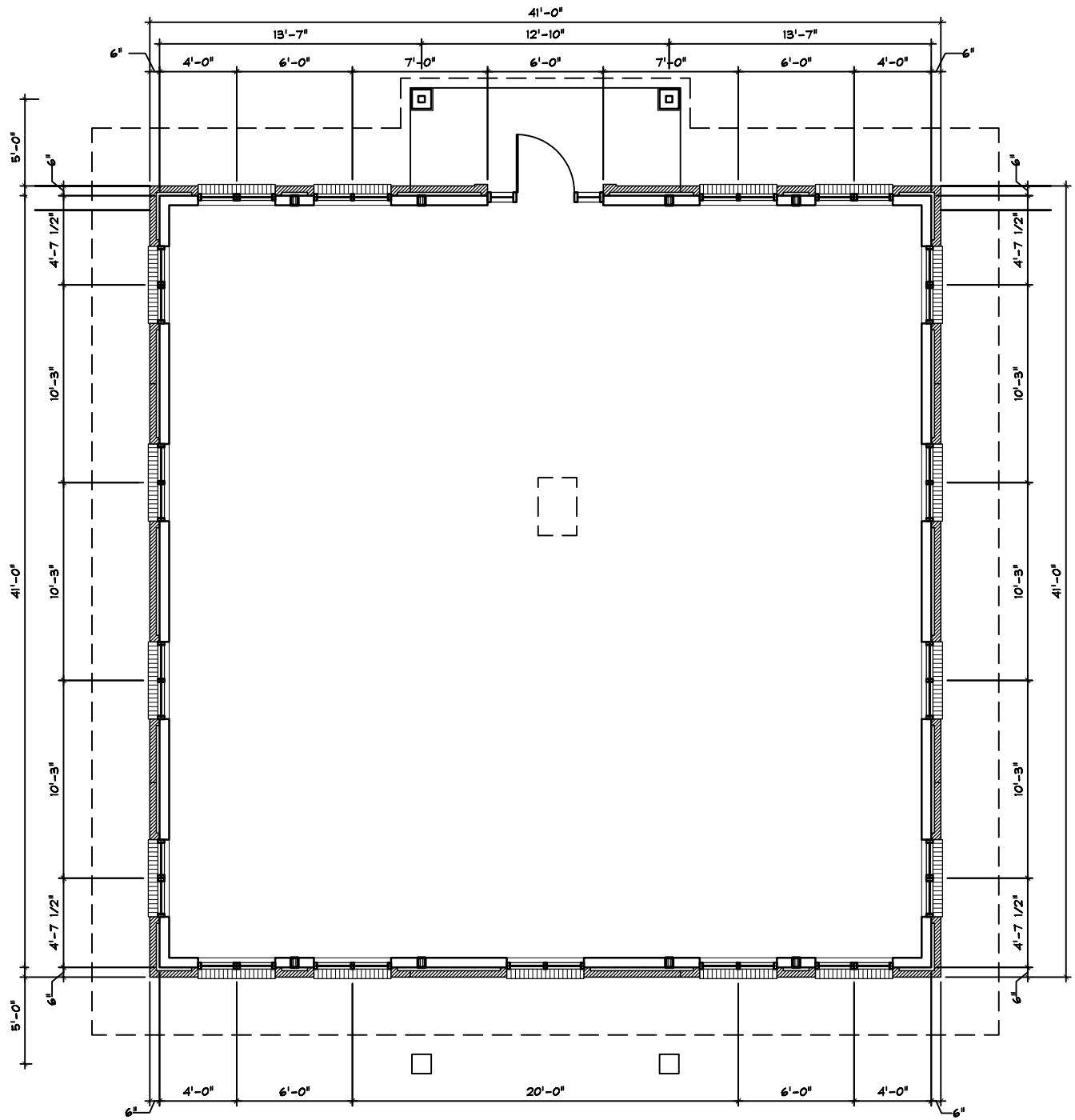
BUILDING B PLAN- UPPER LEVEL (1,600 SQUARE FEET)
