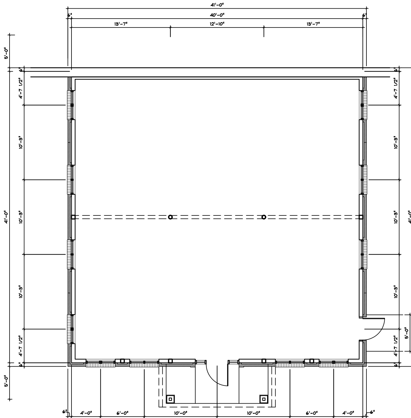
BUILDING B PLAN- LOWER LEVEL (1,600 SQUARE FEET)
