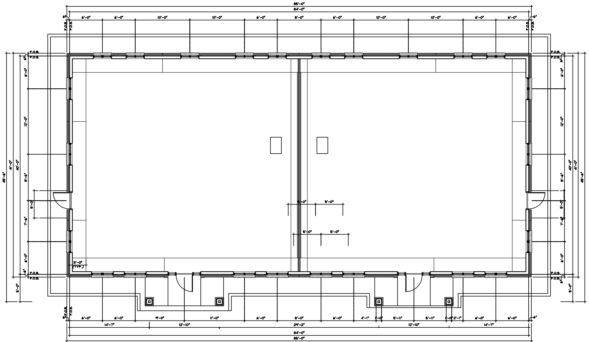
BUILDING A PLAN (3,486 SQUARE FEET)
